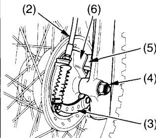
LEFT FRONT
