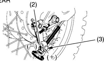
(2) adjusting nut (3) brake arm pin
