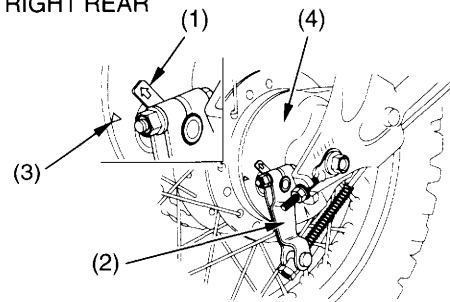
RIGHT REAR
